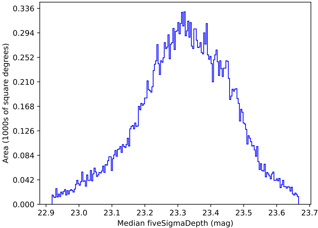
too_elab_r64_d2_griz_v3.4_10yrs All sky all bands: Median fiveSigmaDepth
