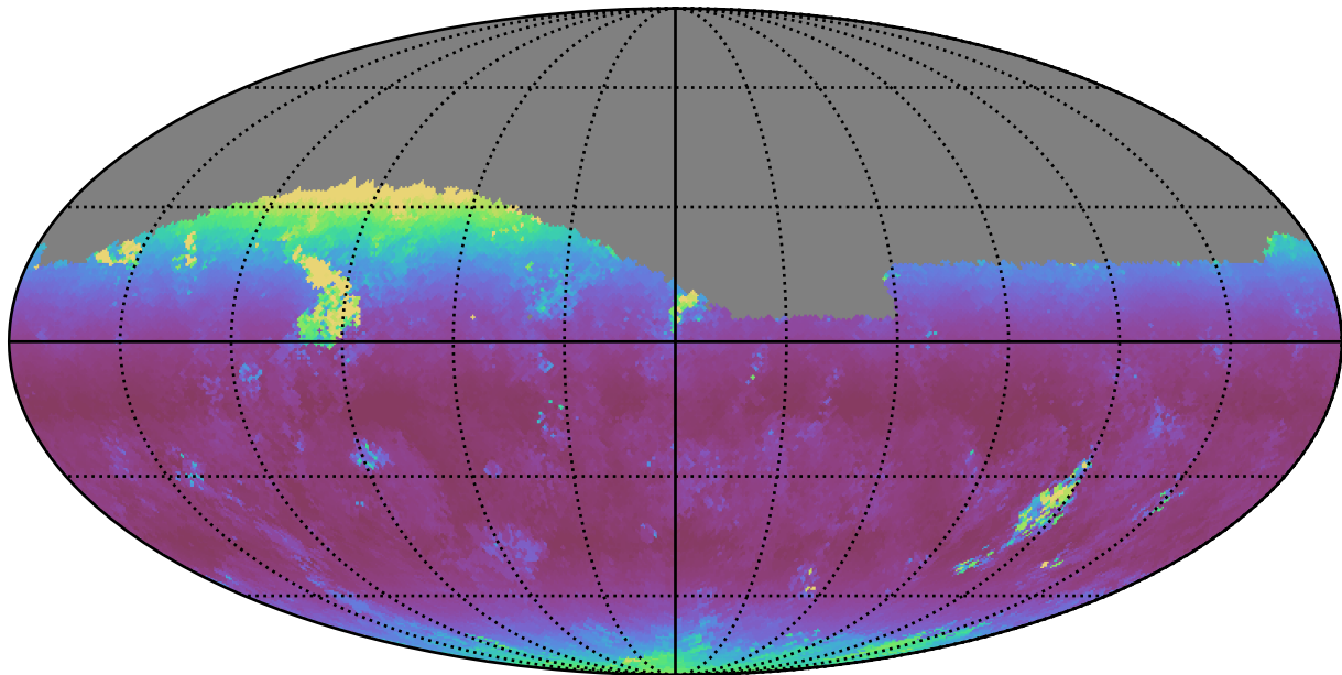
too_elab_r64_d2_griz_v3.4_10yrs Yr 1 z band: Median airmass
