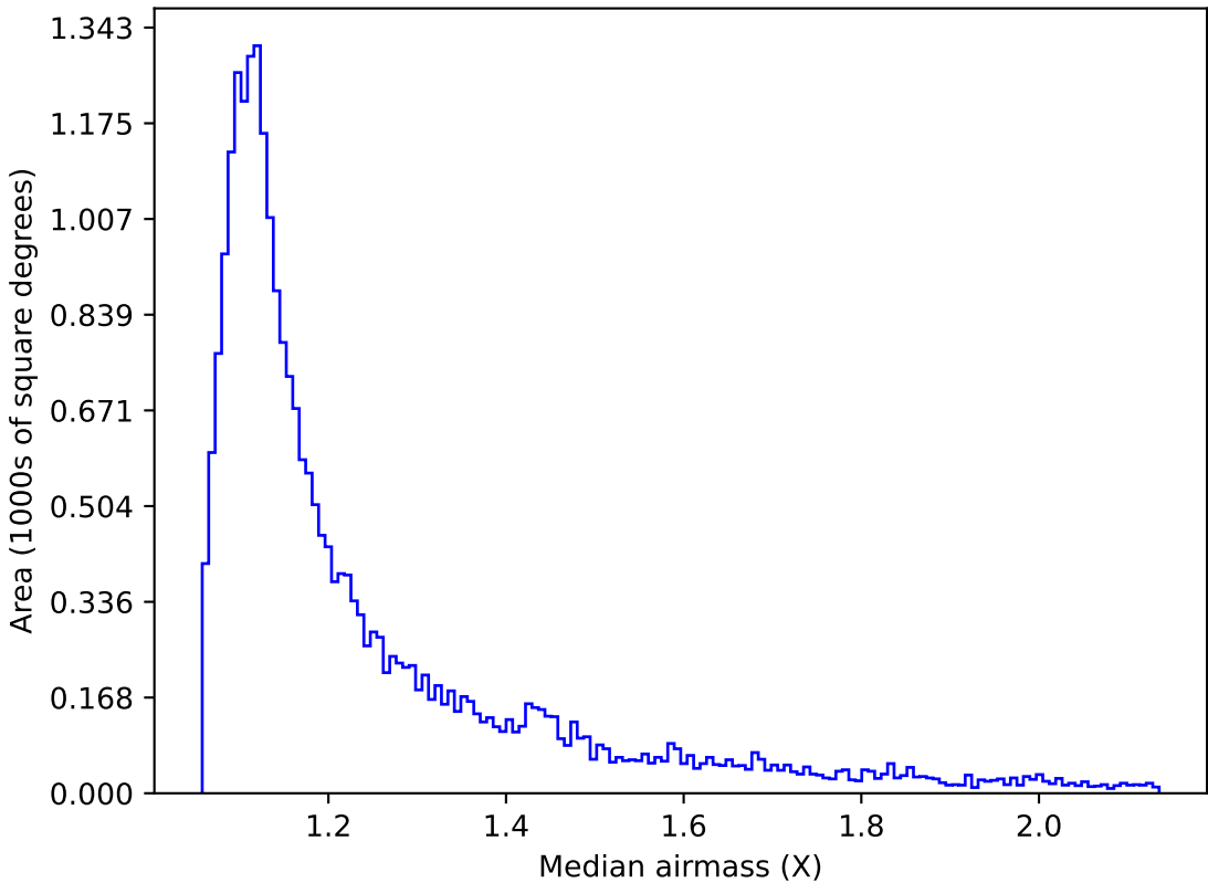
too_elab_r64_d2_griz_v3.4_10yrs Yr 1 r band: Median airmass
