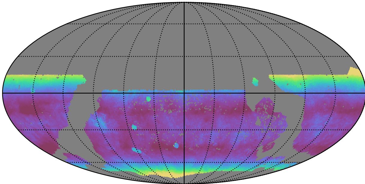
too_elab_r64_d2_griz_v3.4_10yrs WFD z band: Median airmass
