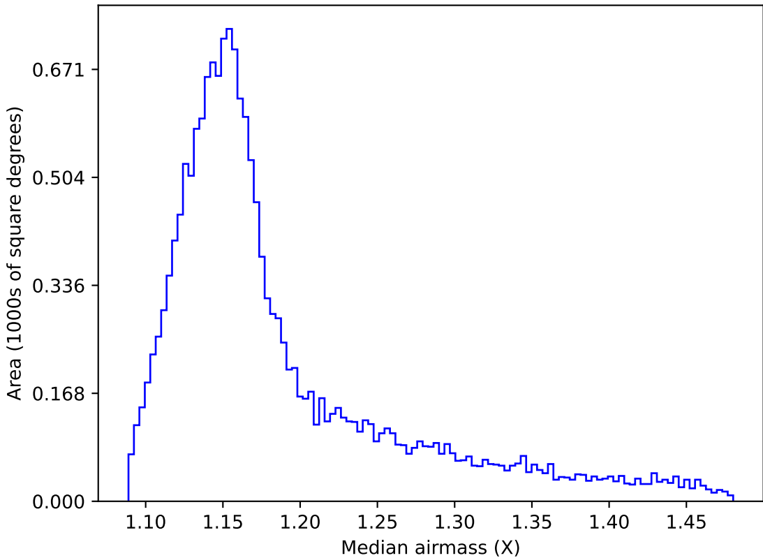
too_elab_r64_d2_griz_v3.4_10yrs WFD z band: Median airmass
