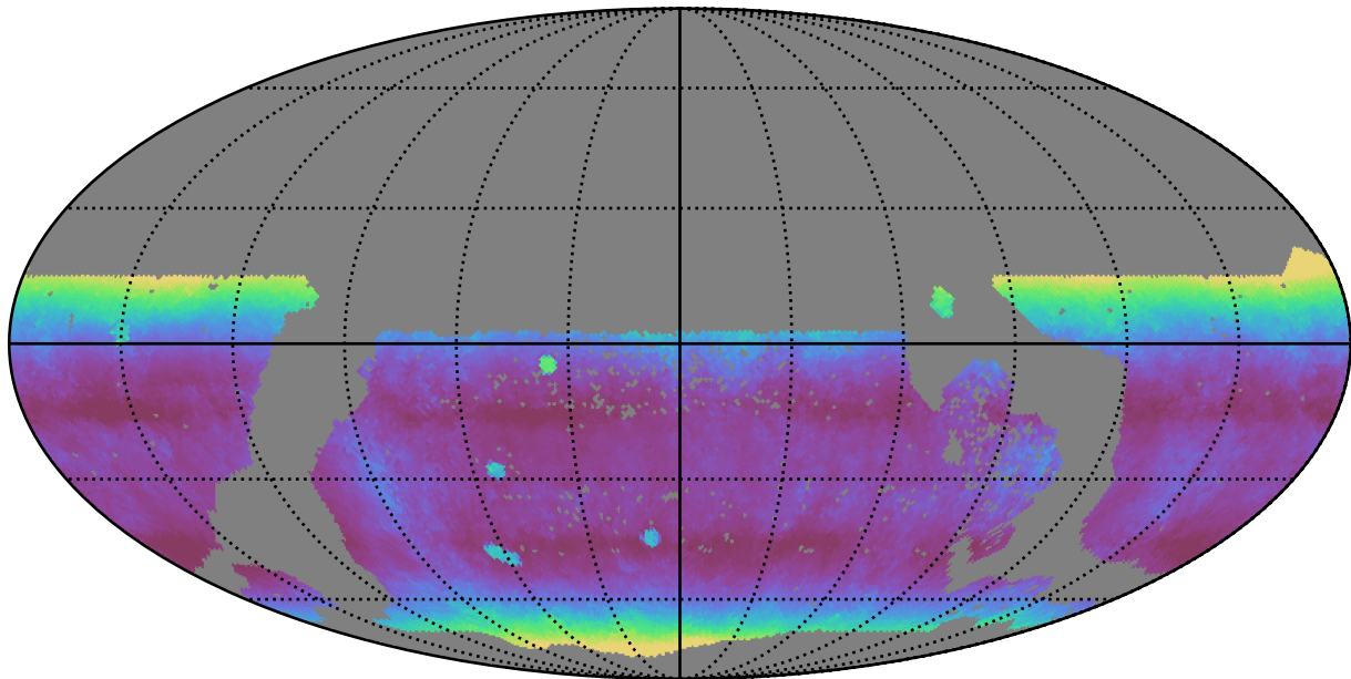
too_elab_r64_d2_griz_v3.4_10yrs WFD y band: Median airmass
