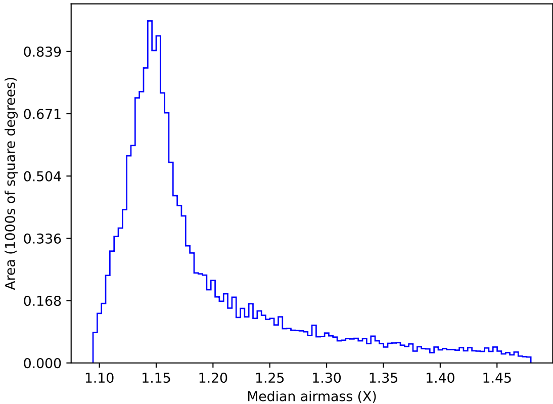
too_elab_r64_d2_griz_v3.4_10yrs WFD y band: Median airmass
