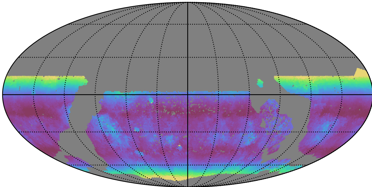
too_elab_r64_d2_griz_v3.4_10yrs WFD u band: Median airmass
