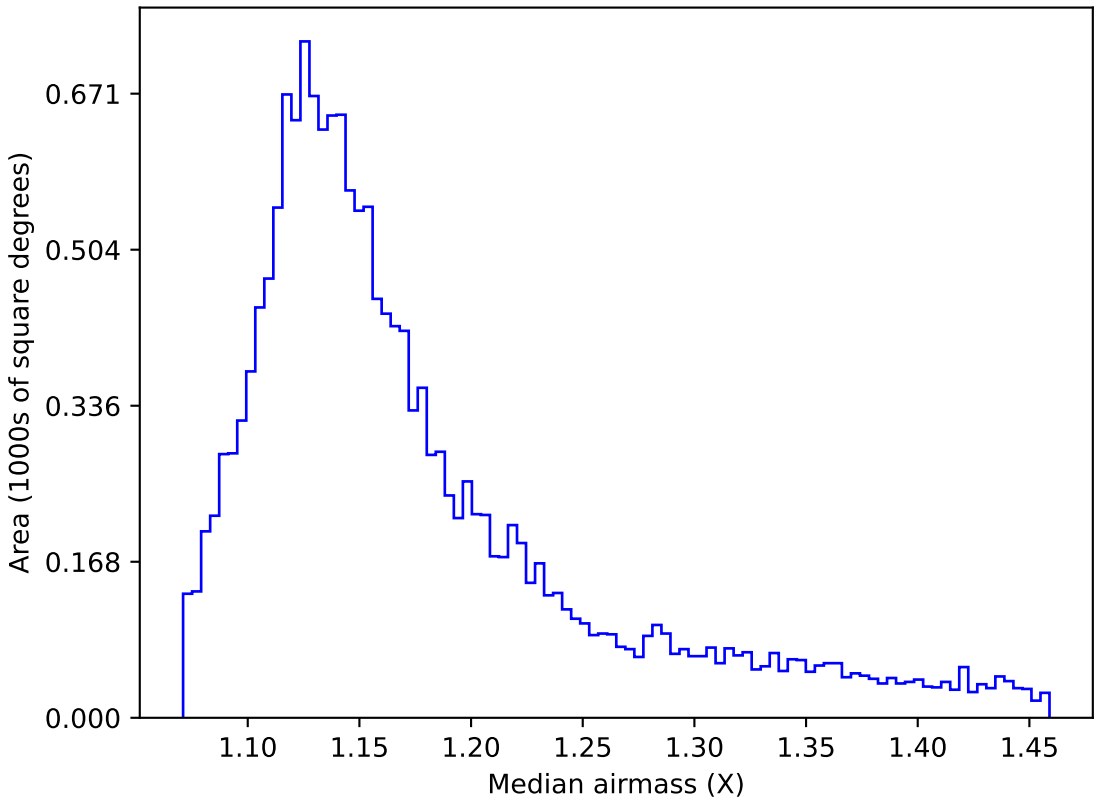
too_elab_r64_d2_griz_v3.4_10yrs WFD u band: Median airmass
