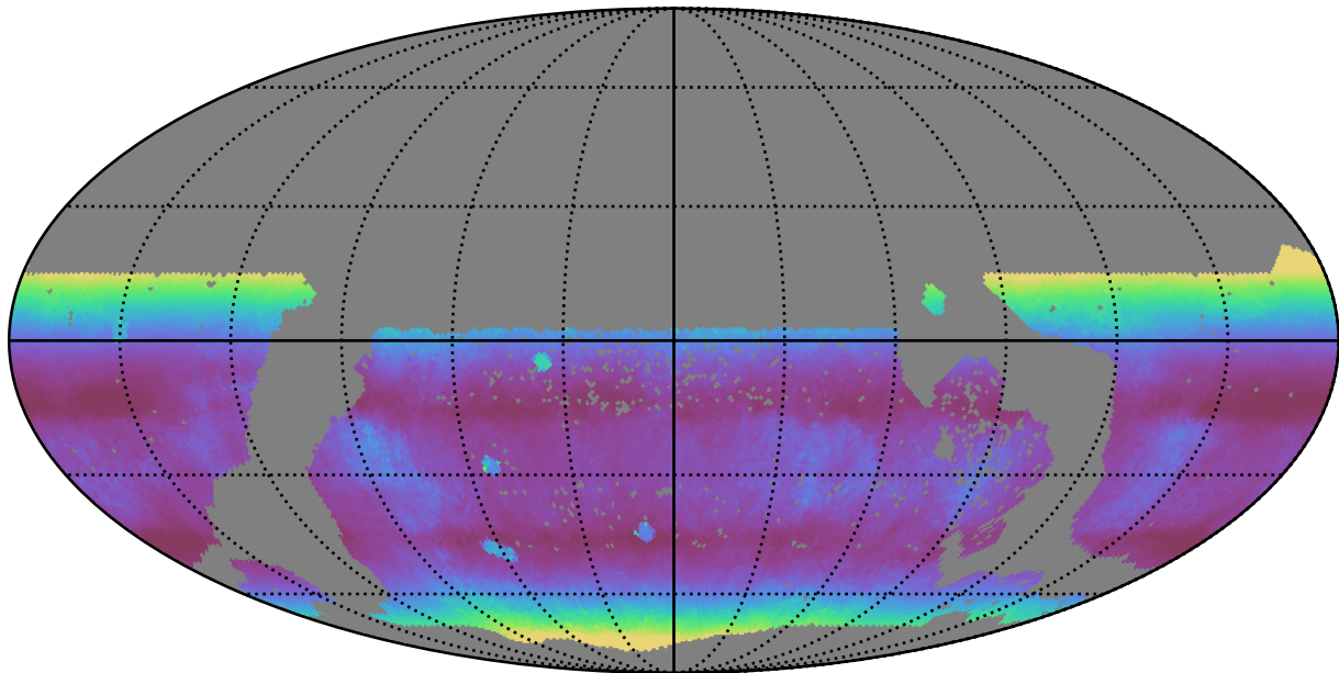
too_elab_r64_d2_griz_v3.4_10yrs WFD r band: Median airmass
