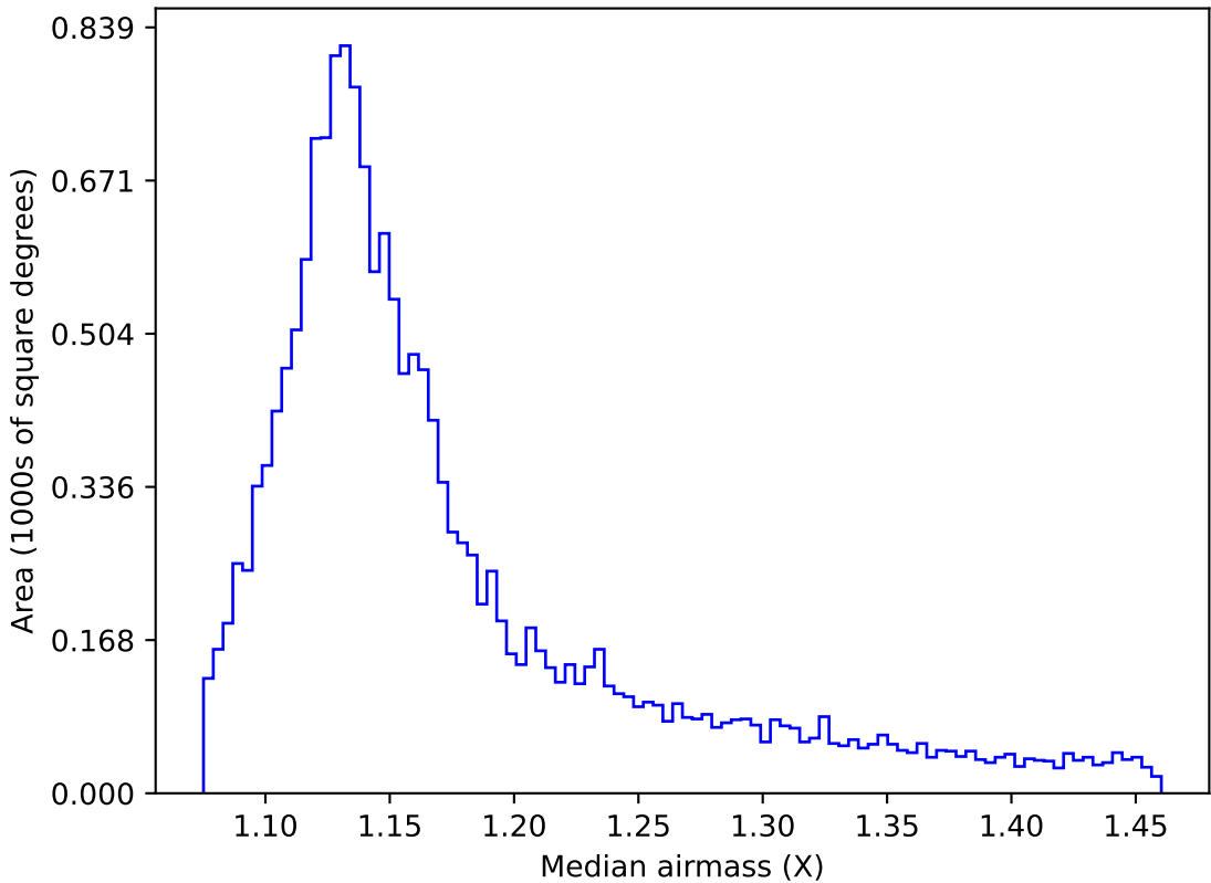
too_elab_r64_d2_griz_v3.4_10yrs WFD r band: Median airmass
