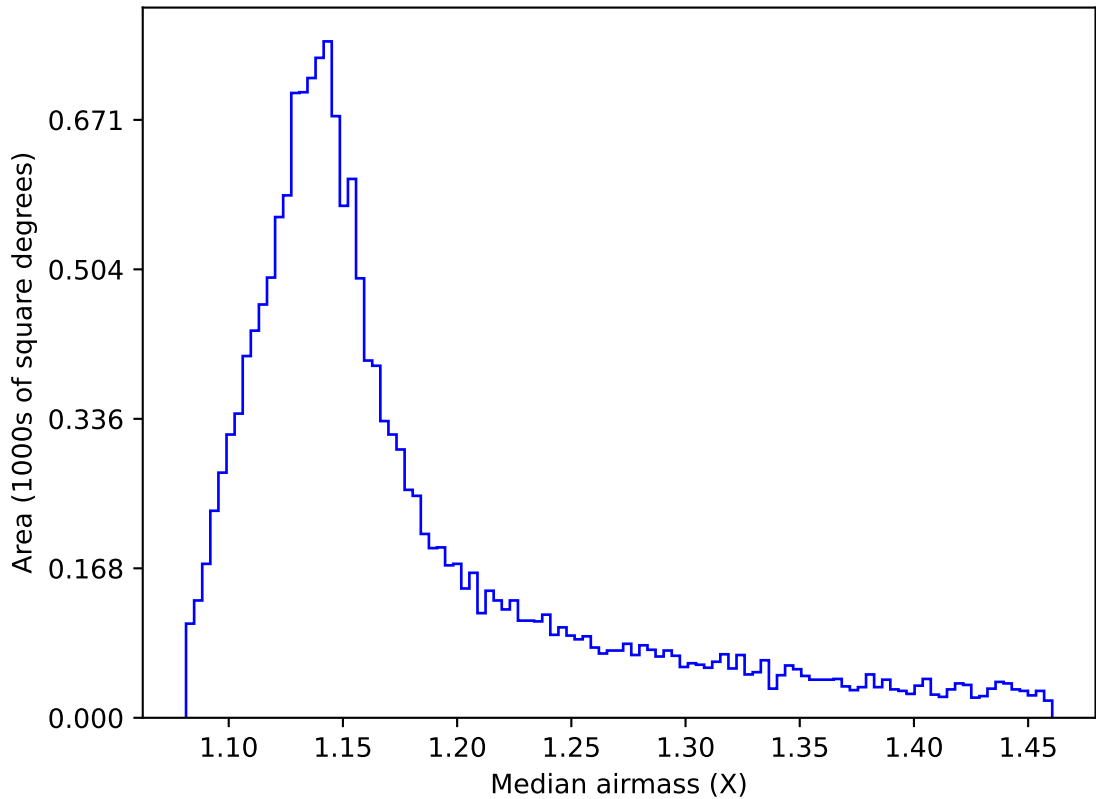
too_elab_r64_d2_griz_v3.4_10yrs WFD i band: Median airmass
