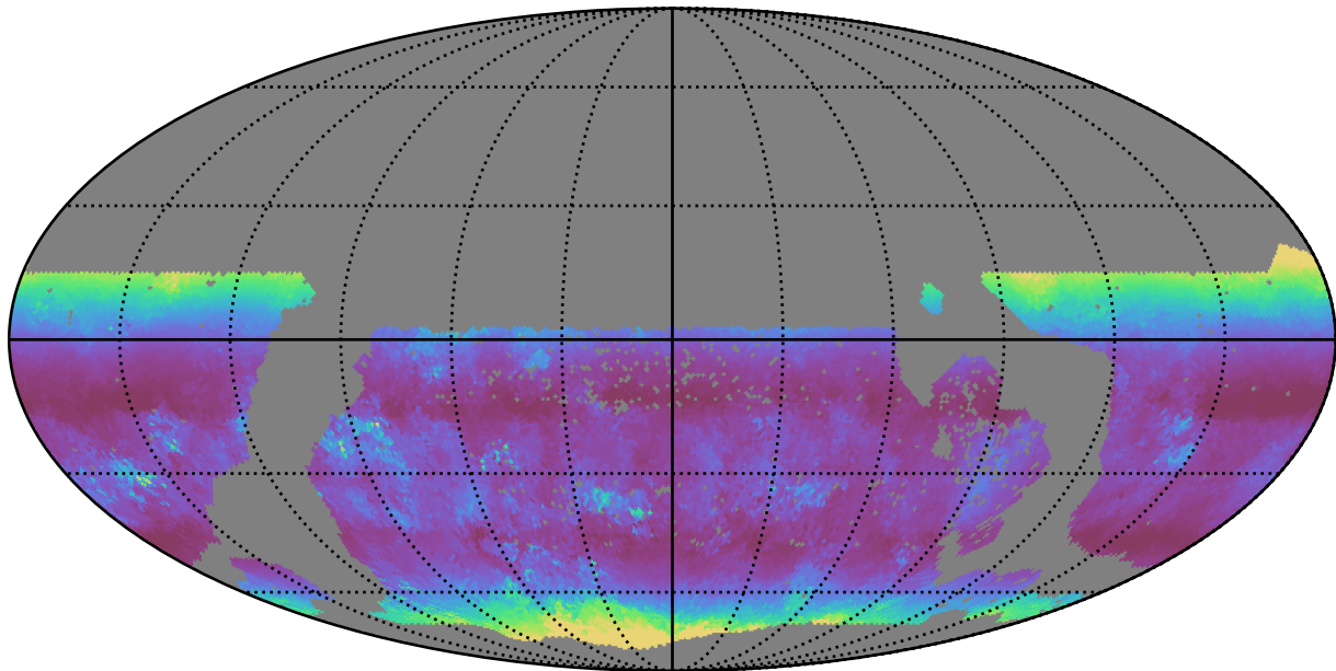
too_elab_r64_d2_griz_v3.4_10yrs WFD g band: Median airmass
