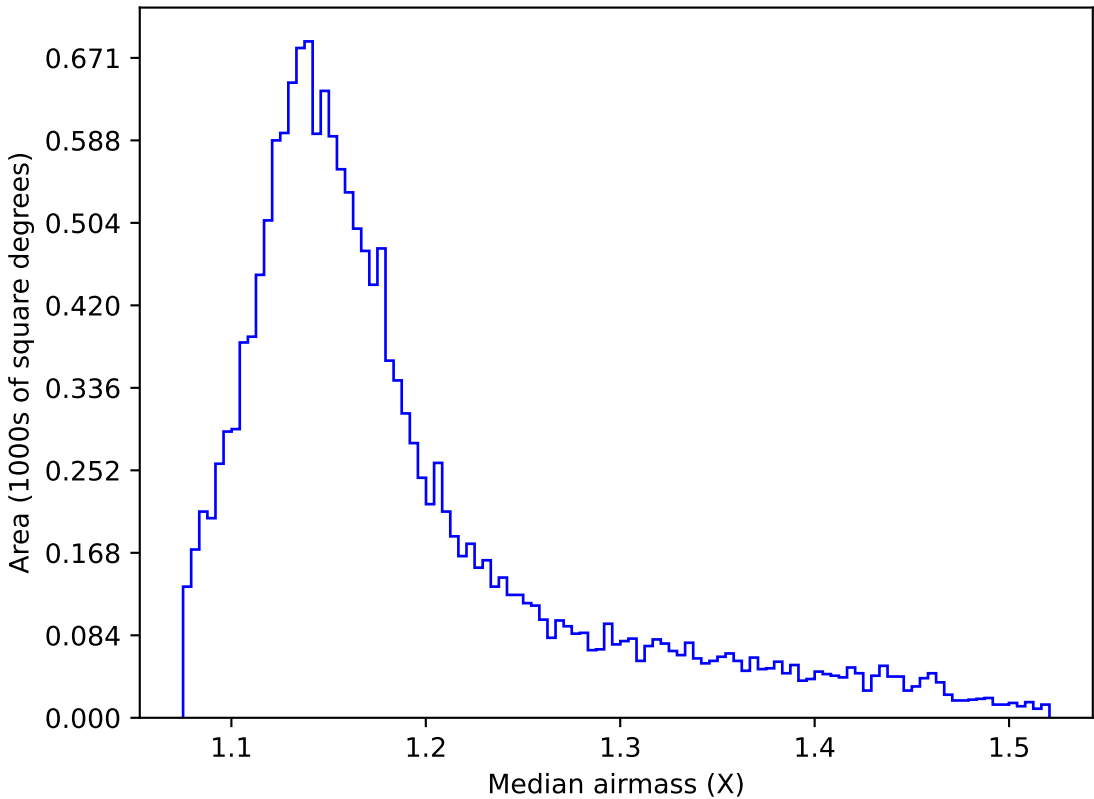
too_elab_r64_d2_griz_v3.4_10yrs WFD g band: Median airmass
