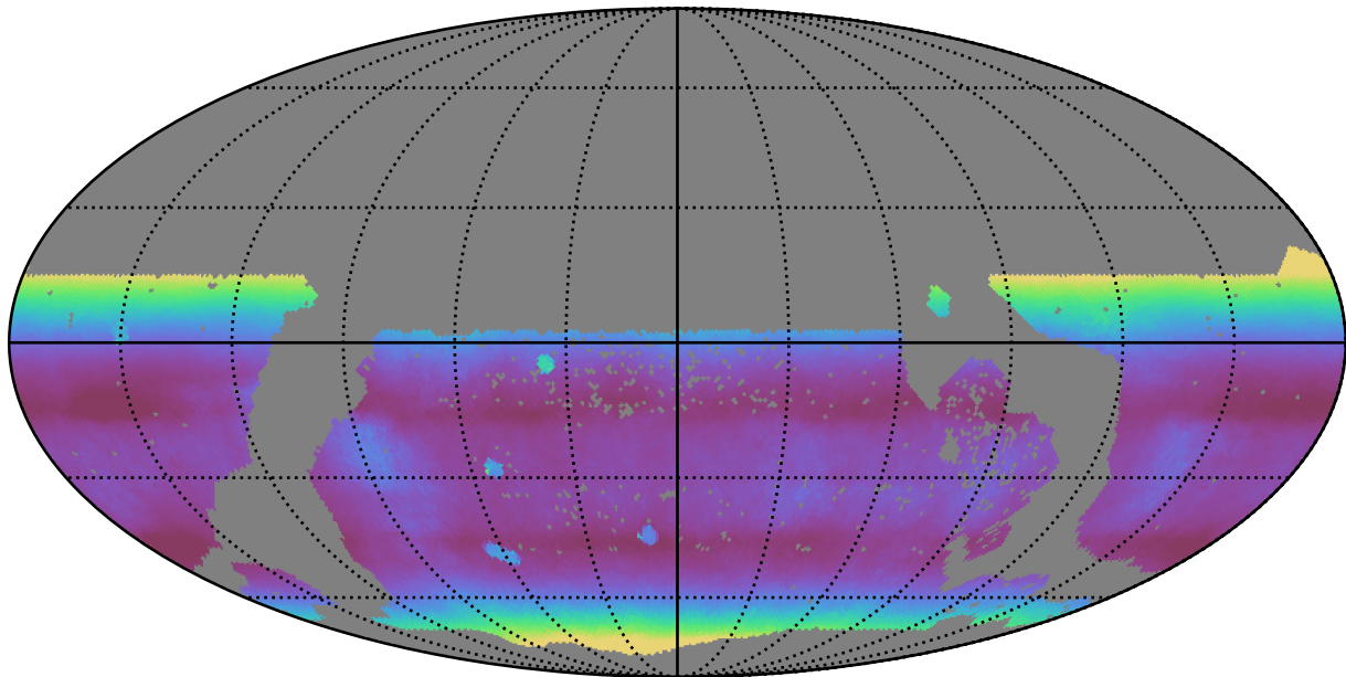
too_elab_r64_d2_griz_v3.4_10yrs WFD all bands: Median airmass
