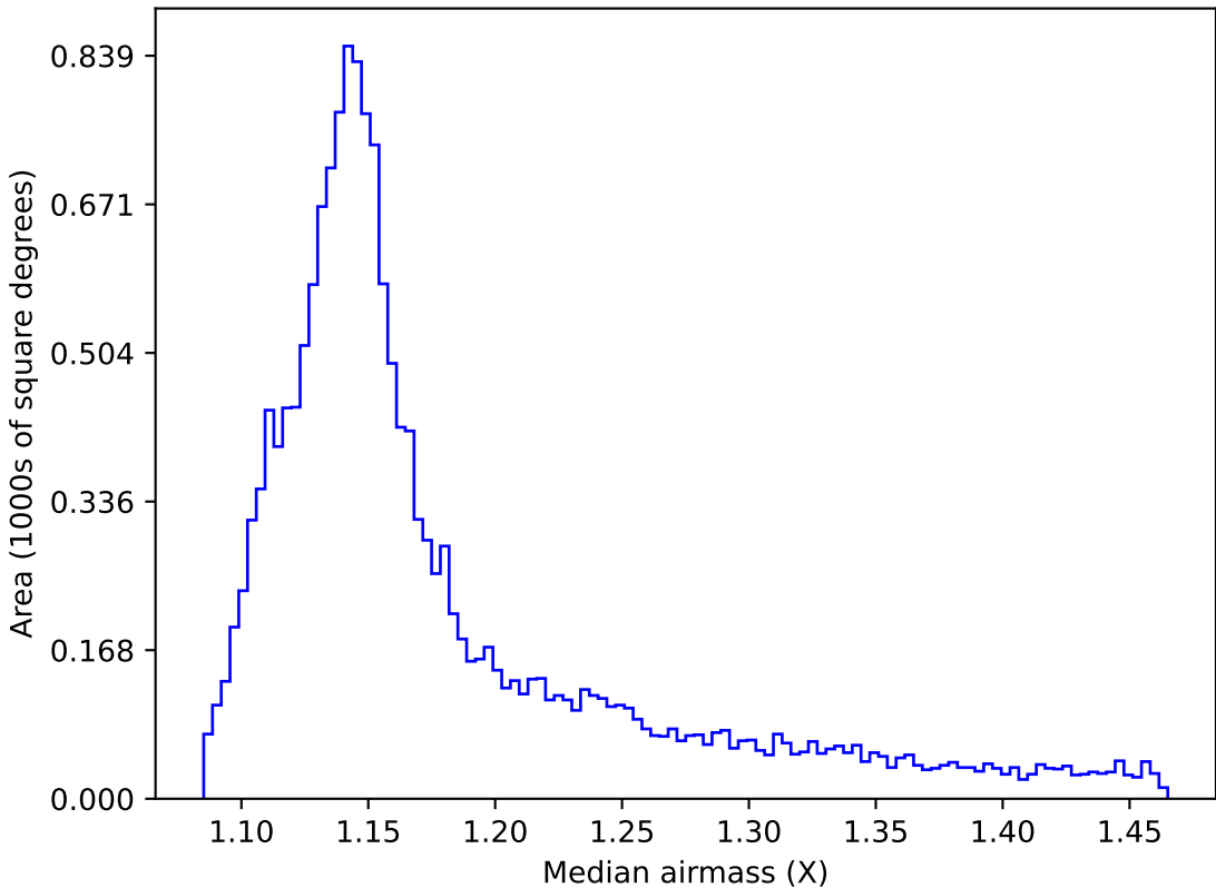
too_elab_r64_d2_griz_v3.4_10yrs WFD all bands: Median airmass
