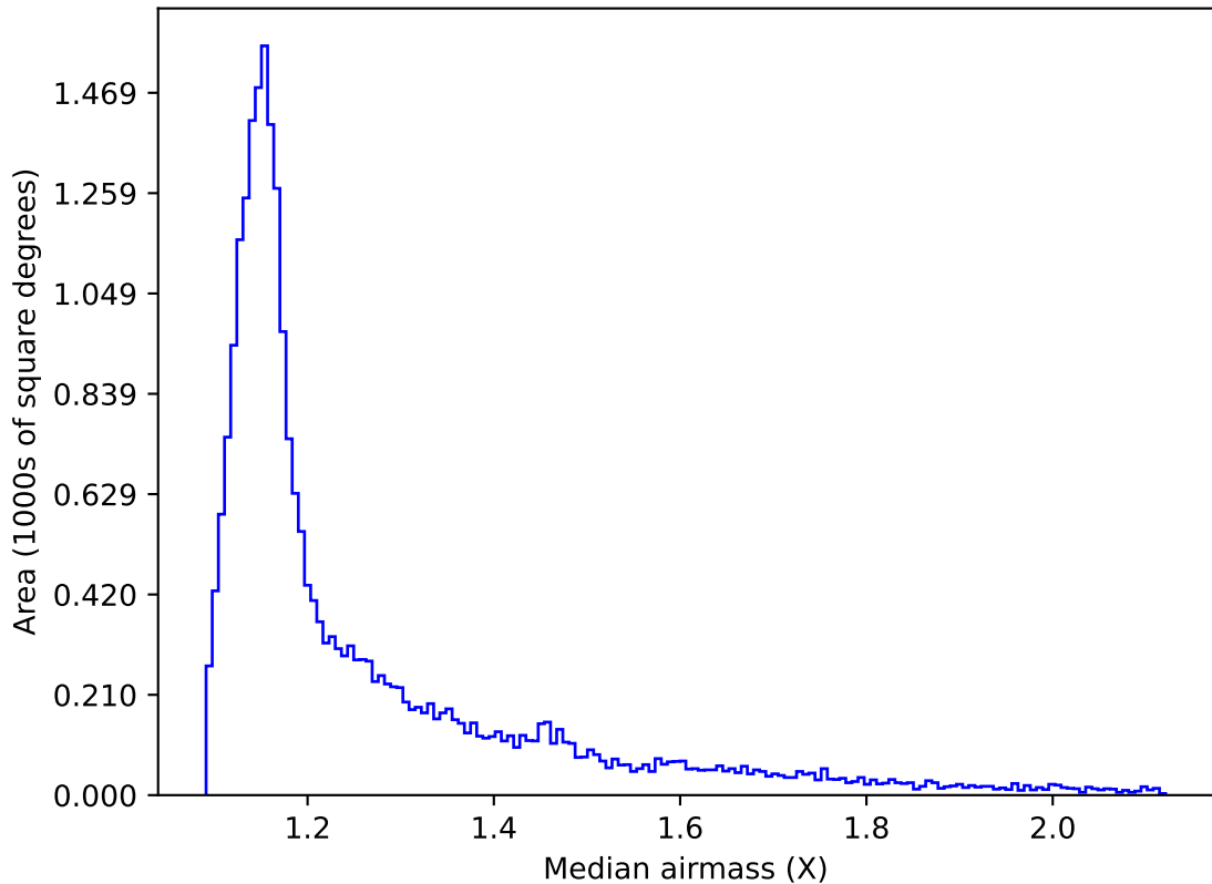
too_elab_r64_d2_griz_v3.4_10yrs All sky z band: Median airmass
