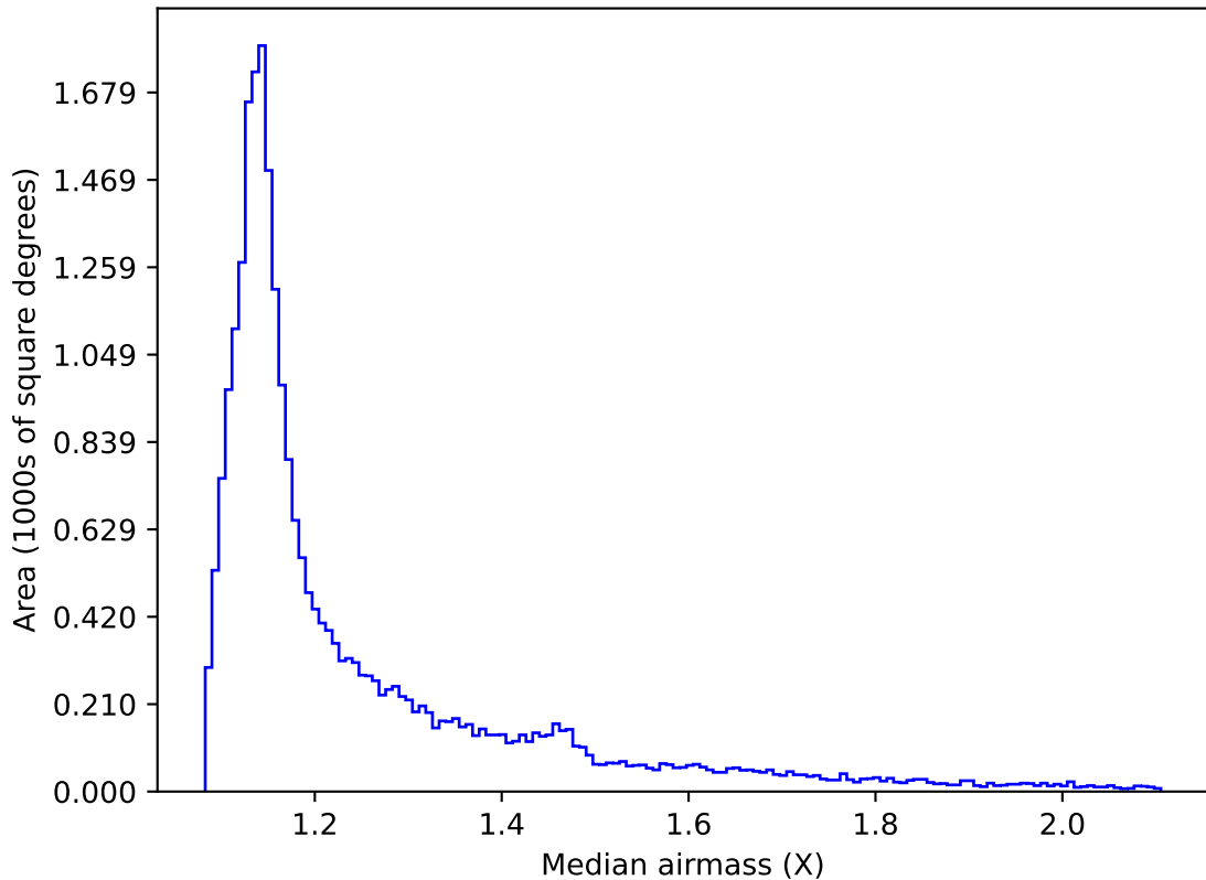
too_elab_r64_d2_griz_v3.4_10yrs All sky i band: Median airmass
