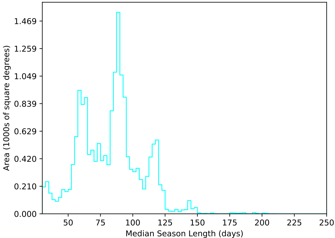
too_elab_r64_d2_griz_v3.4_10yrs WFD u band: Median Season Length
