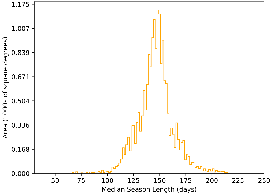
too_elab_r64_d2_griz_v3.4_10yrs WFD r band: Median Season Length
