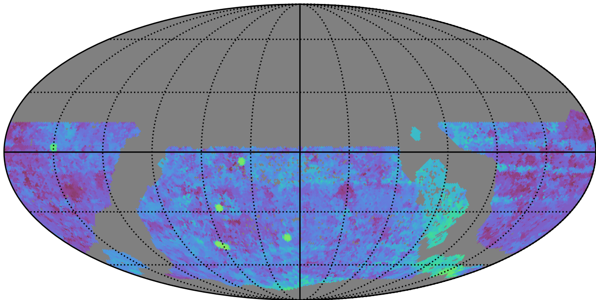
too_elab_r64_d2_griz_v3.4_10yrs WFD g band: Median Season Length
