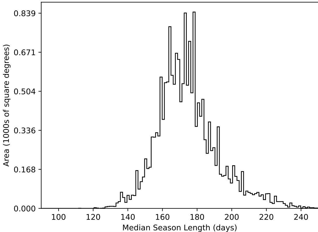
too_elab_r64_d2_griz_v3.4_10yrs WFD all bands: Median Season Length
