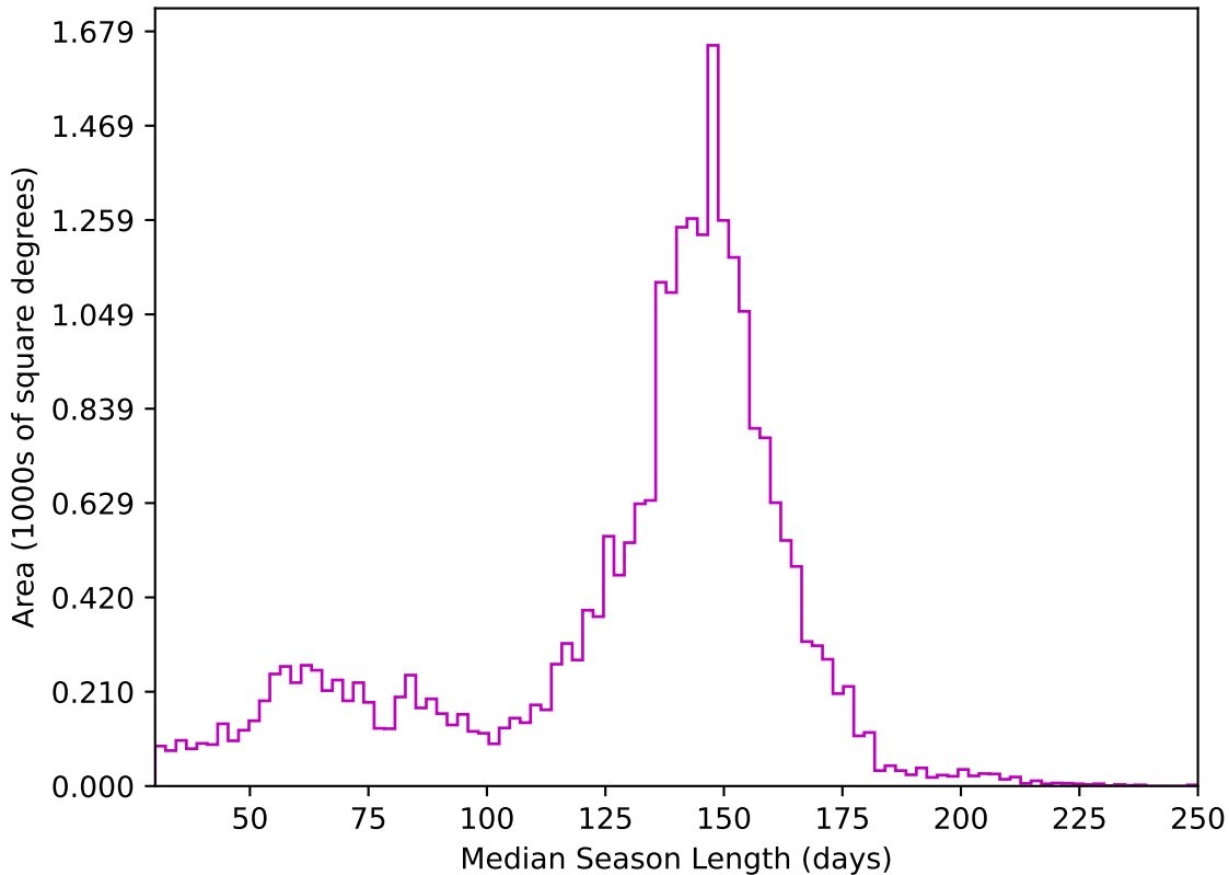
too_elab_r64_d2_griz_v3.4_10yrs All sky z band: Median Season Length
