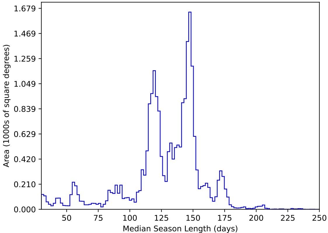
too_elab_r64_d2_griz_v3.4_10yrs All sky y band: Median Season Length
