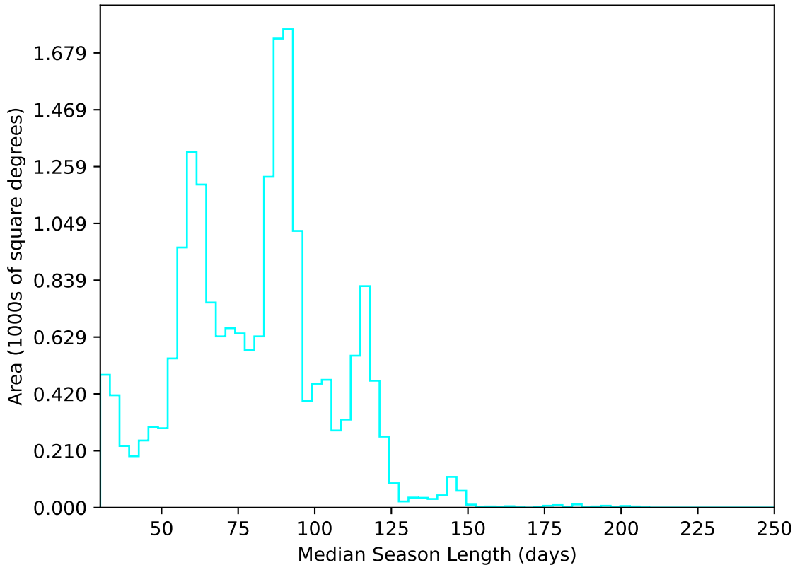
too_elab_r64_d2_griz_v3.4_10yrs All sky u band: Median Season Length
