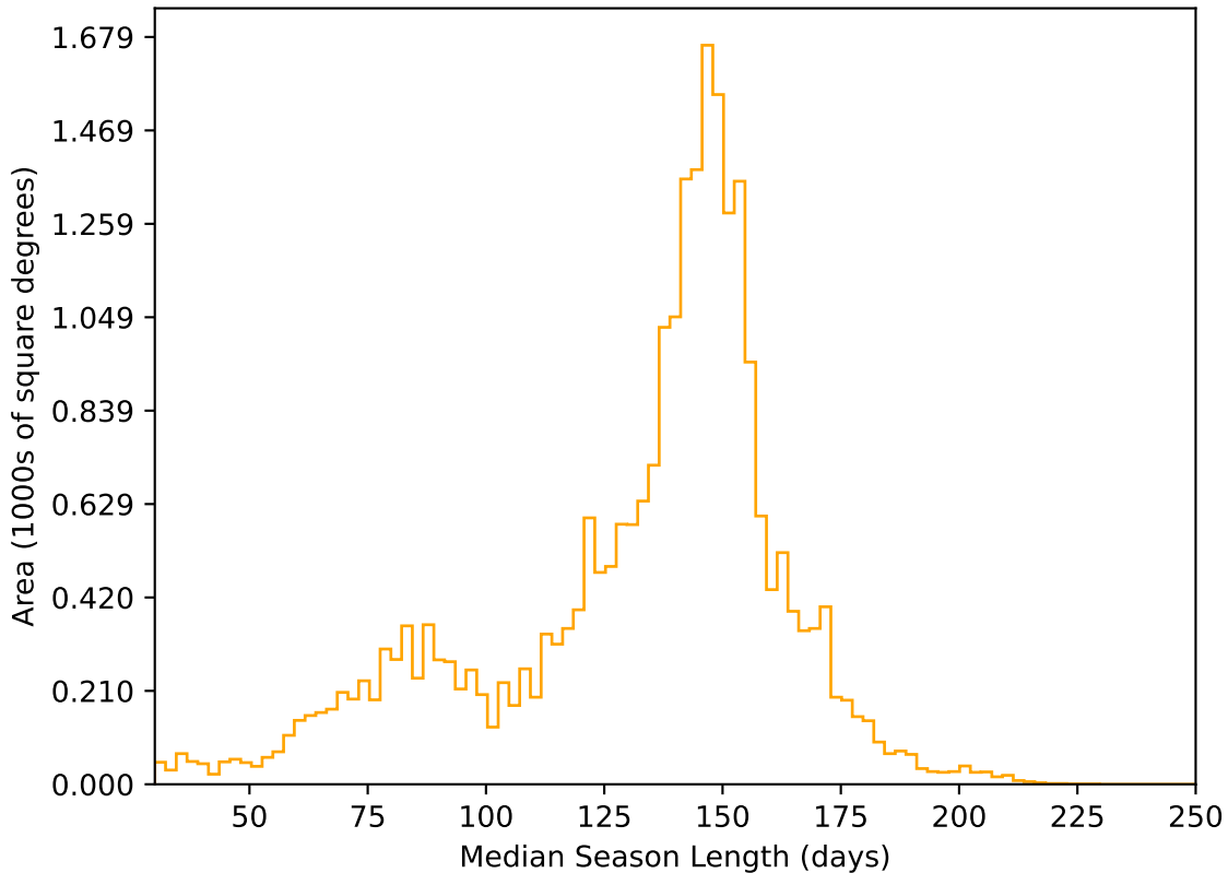
too_elab_r64_d2_griz_v3.4_10yrs All sky r band: Median Season Length
