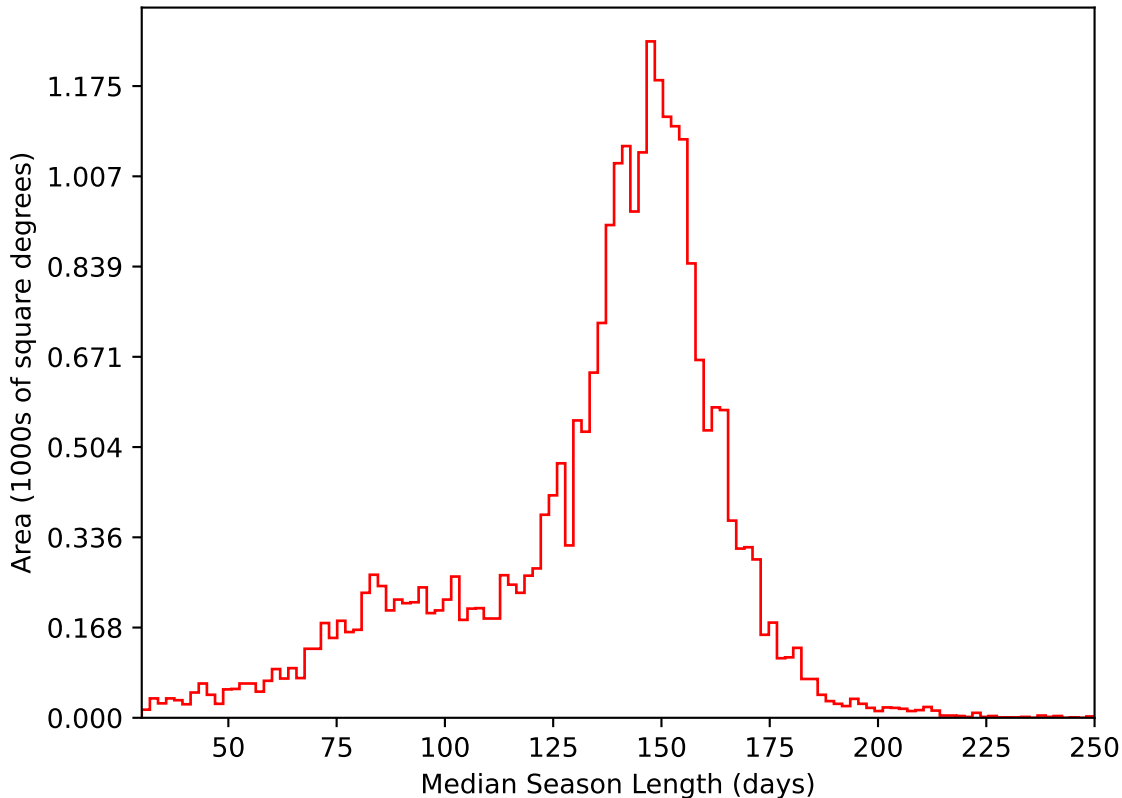
too_elab_r64_d2_griz_v3.4_10yrs All sky i band: Median Season Length
