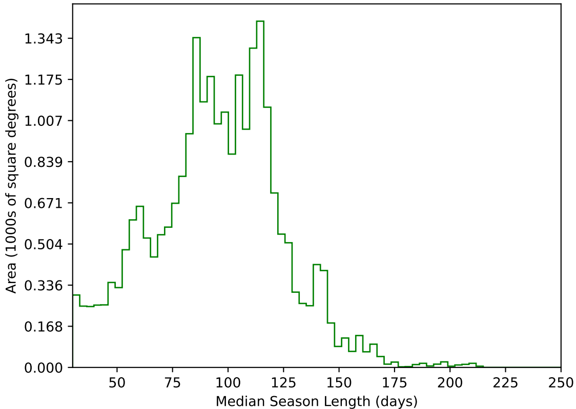
too_elab_r64_d2_griz_v3.4_10yrs All sky g band: Median Season Length
