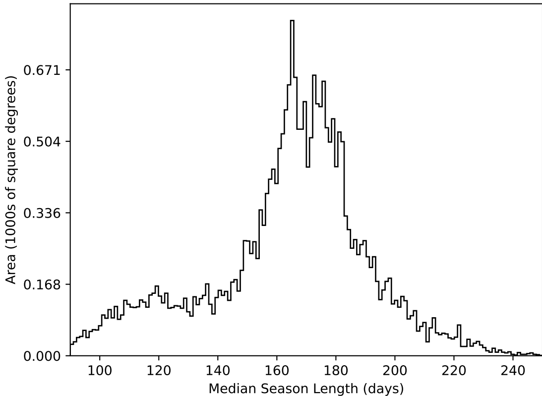
too_elab_r64_d2_griz_v3.4_10yrs All sky all bands: Median Season Length
