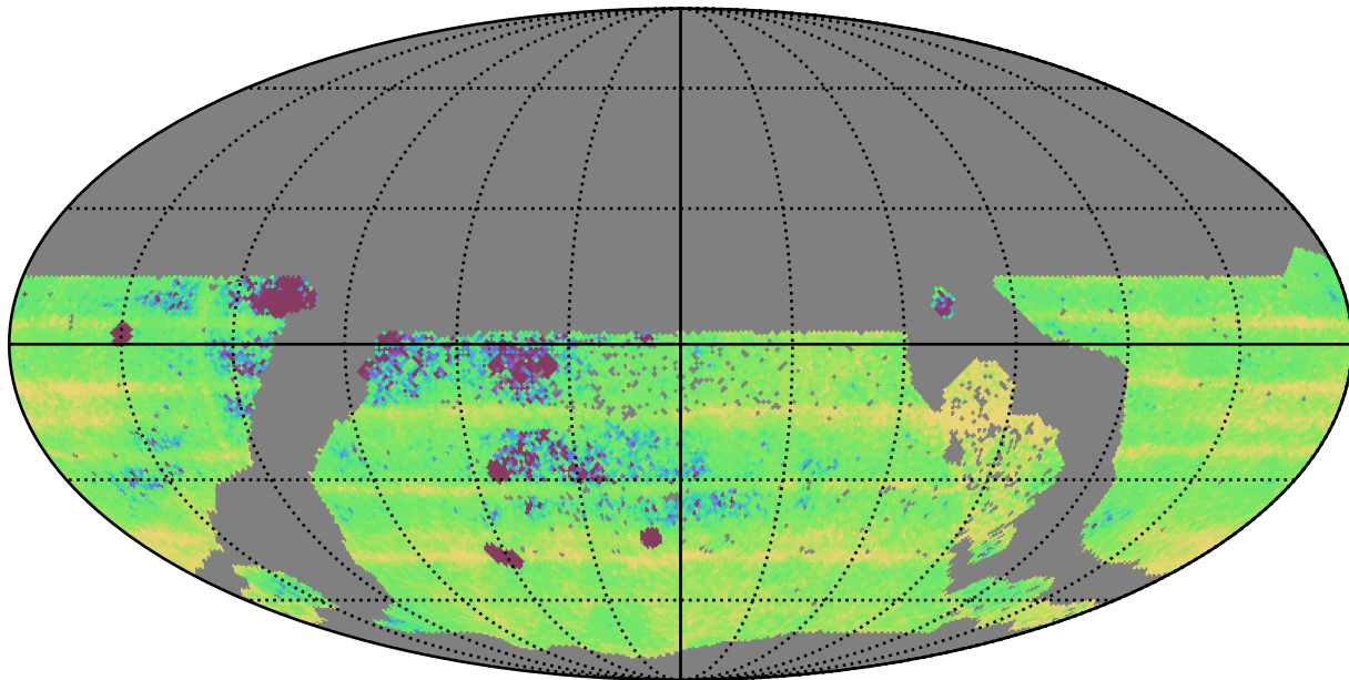
too_elab_r64_d2_griz_v3.4_10yrs WFD: Median Intra-Night Gap
