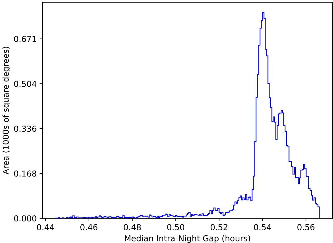
too_elab_r64_d2_griz_v3.4_10yrs WFD: Median Intra-Night Gap
