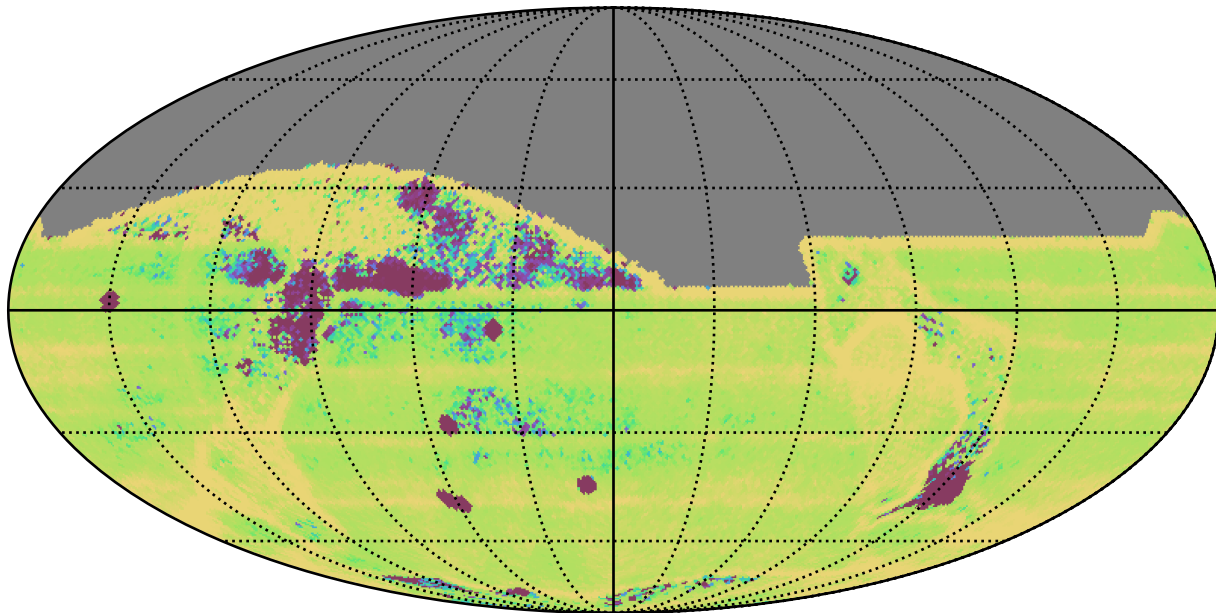
too_elab_r64_d2_griz_v3.4_10yrs All sky: Median Intra-Night Gap
