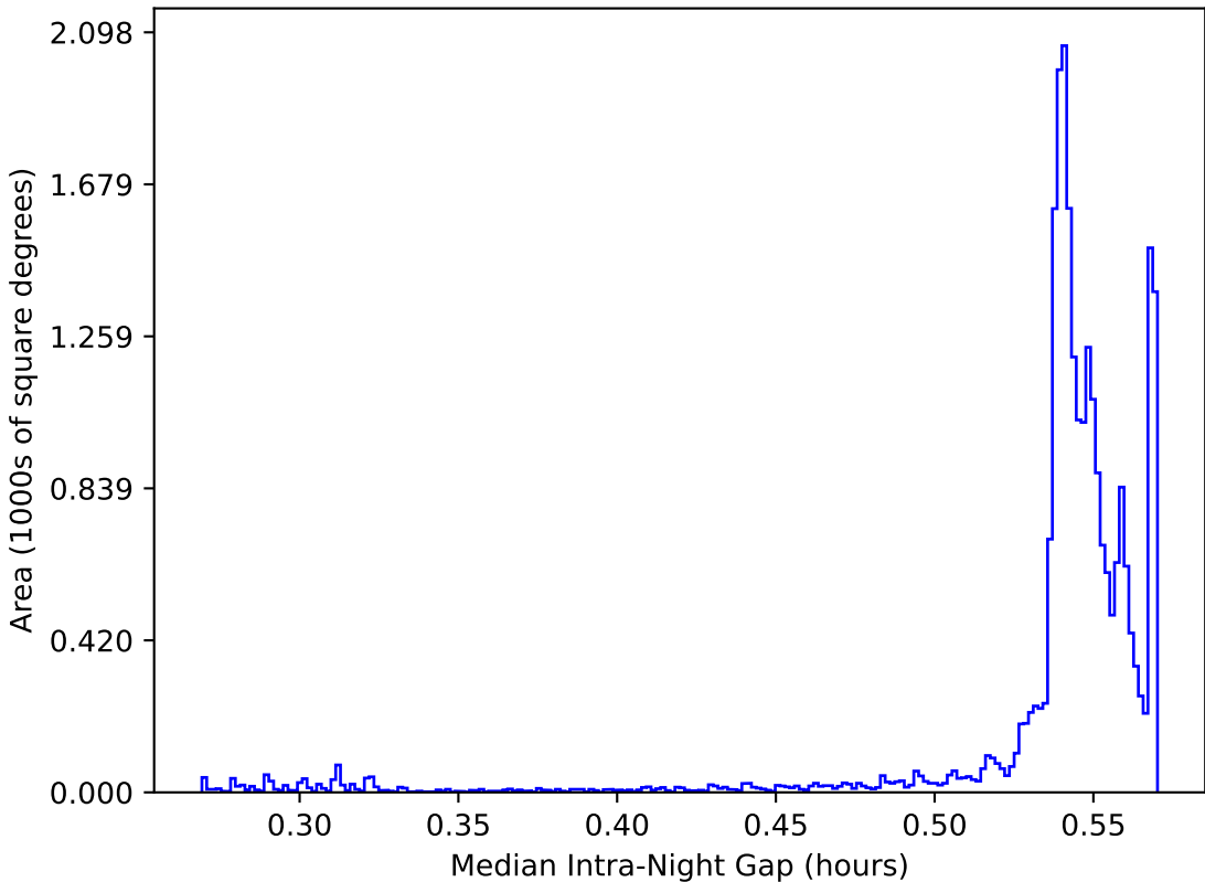
too_elab_r64_d2_griz_v3.4_10yrs All sky: Median Intra-Night Gap
