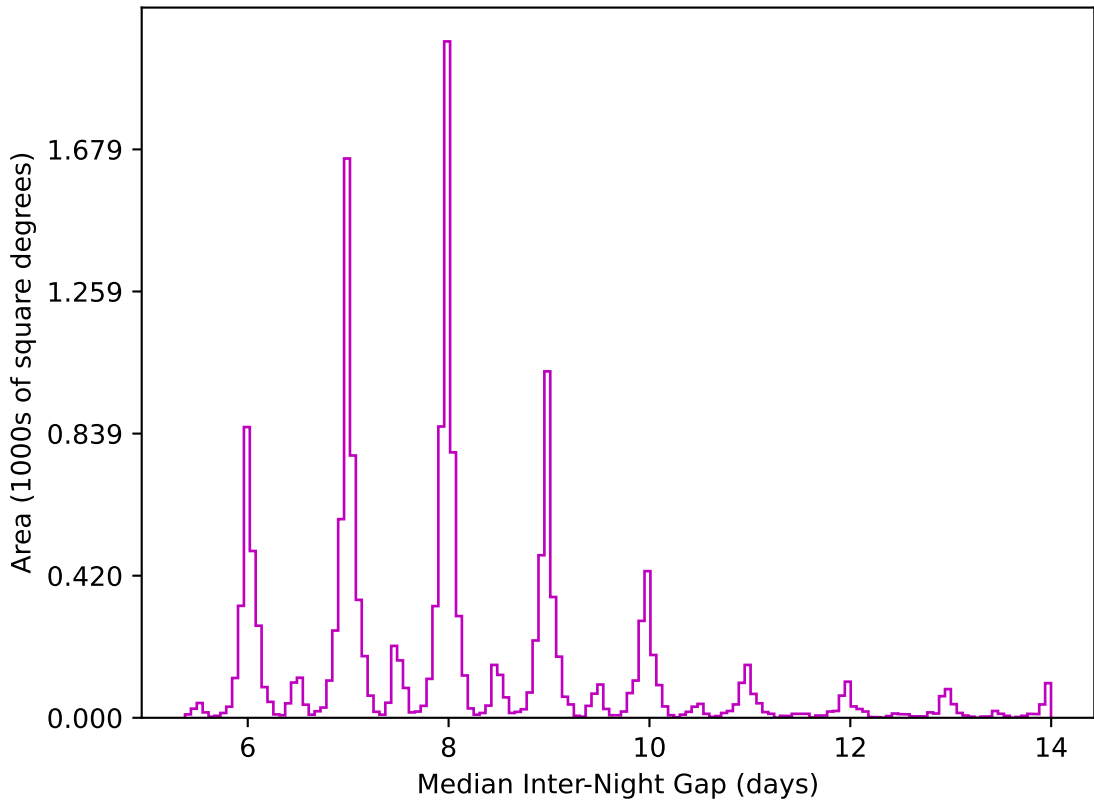
too_elab_r64_d2_griz_v3.4_10yrs WFD z band: Median Inter-Night Gap
