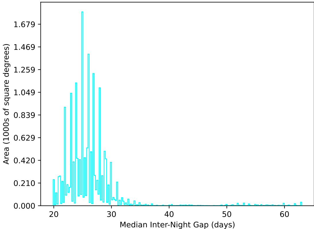
too_elab_r64_d2_griz_v3.4_10yrs WFD u band: Median Inter-Night Gap
