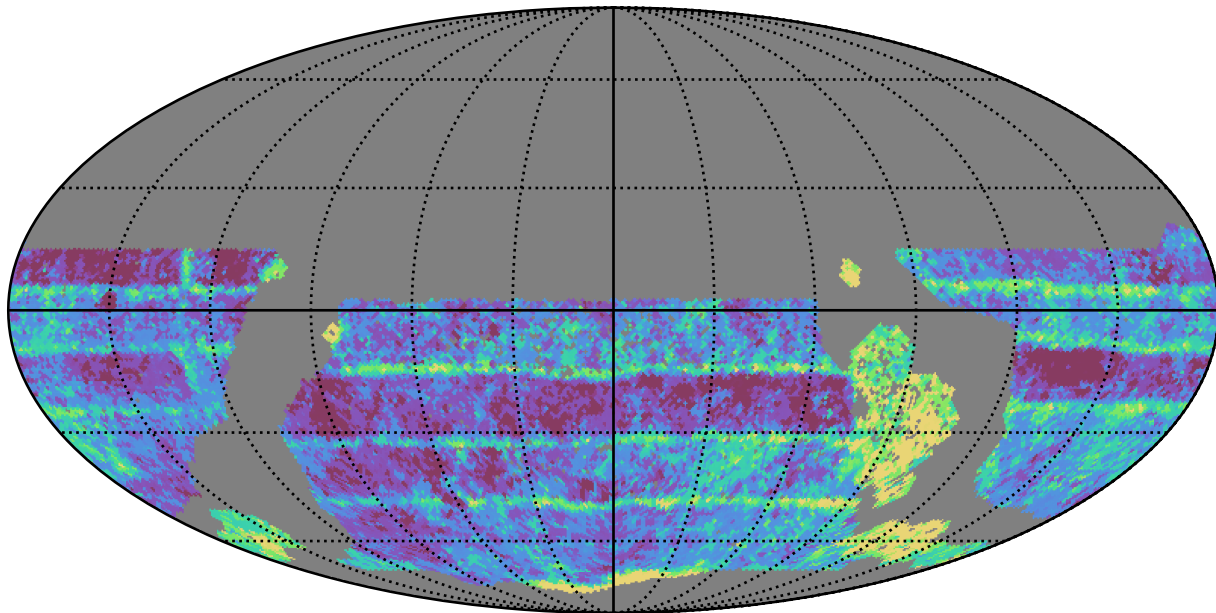
too_elab_r64_d2_griz_v3.4_10yrs WFD i band: Median Inter-Night Gap
