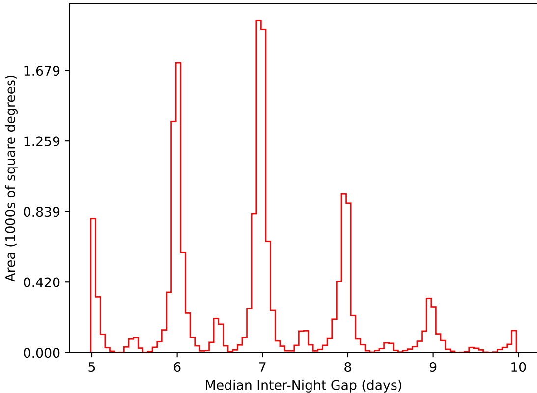
too_elab_r64_d2_griz_v3.4_10yrs WFD i band: Median Inter-Night Gap
