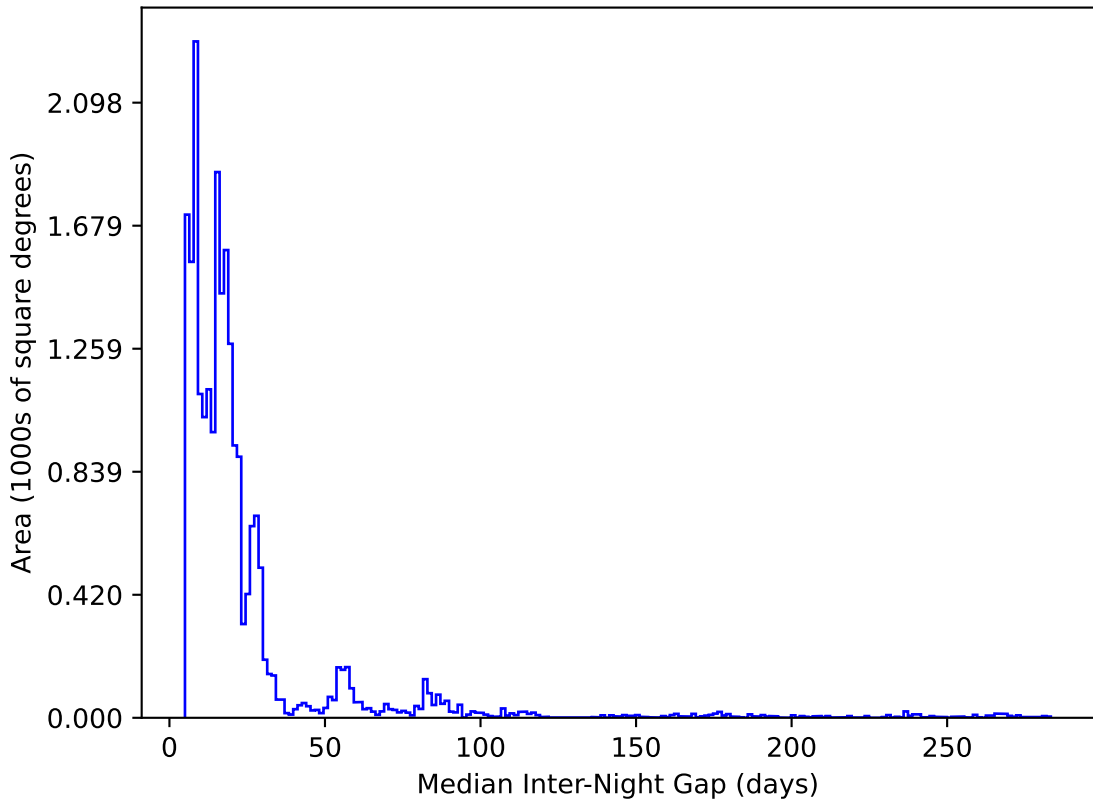
too_elab_r64_d2_griz_v3.4_10yrs All sky y band: Median Inter-Night Gap
