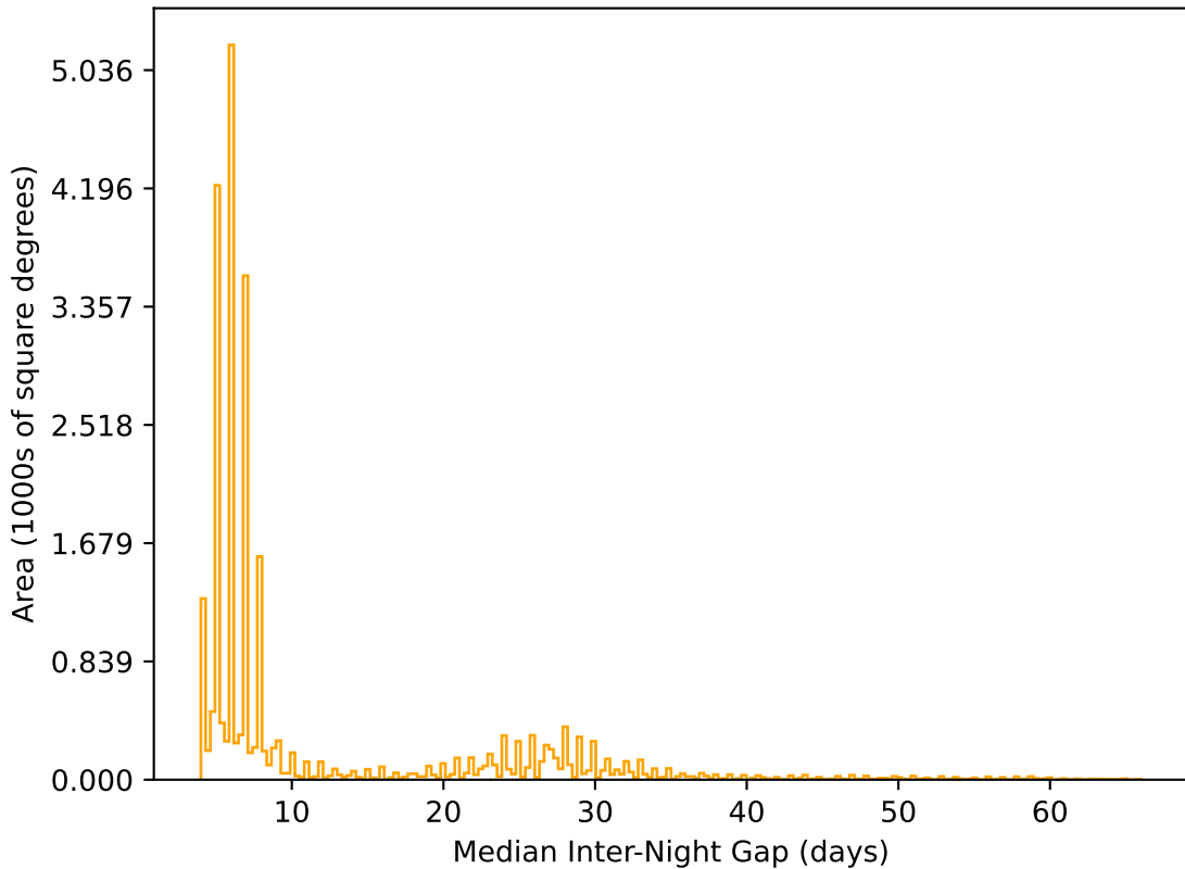
too_elab_r64_d2_griz_v3.4_10yrs All sky r band: Median Inter-Night Gap
