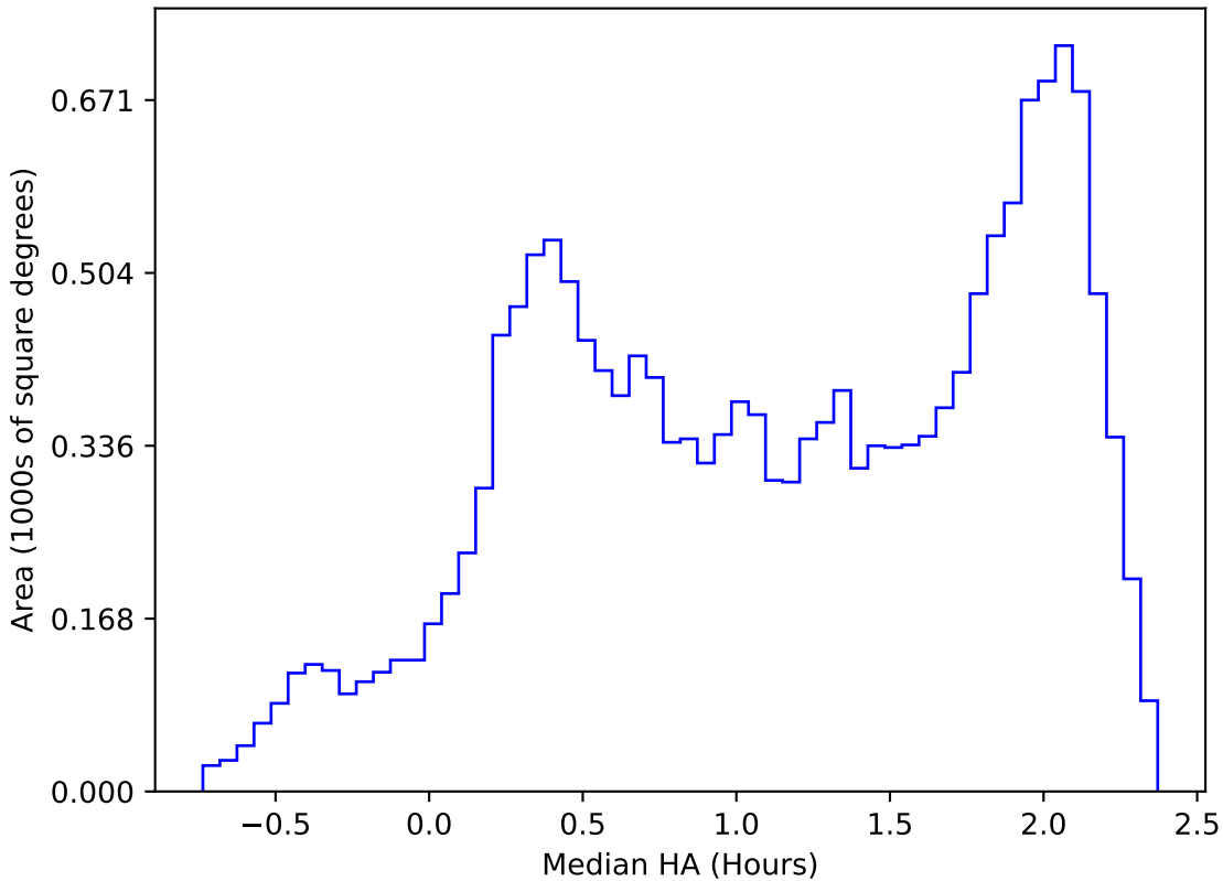
too_elab_r64_d2_griz_v3.4_10yrs WFD z band: Median HA
