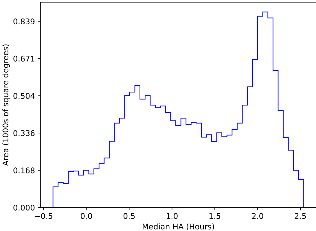
too_elab_r64_d2_griz_v3.4_10yrs WFD y band: Median HA
