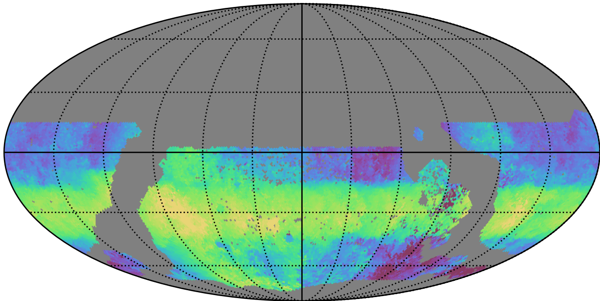
too_elab_r64_d2_griz_v3.4_10yrs WFD u band: Median HA
