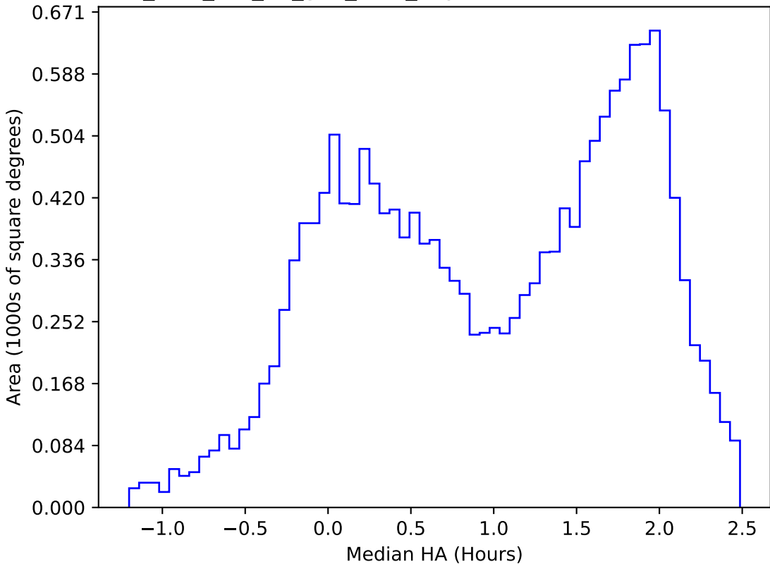
too_elab_r64_d2_griz_v3.4_10yrs WFD u band: Median HA
