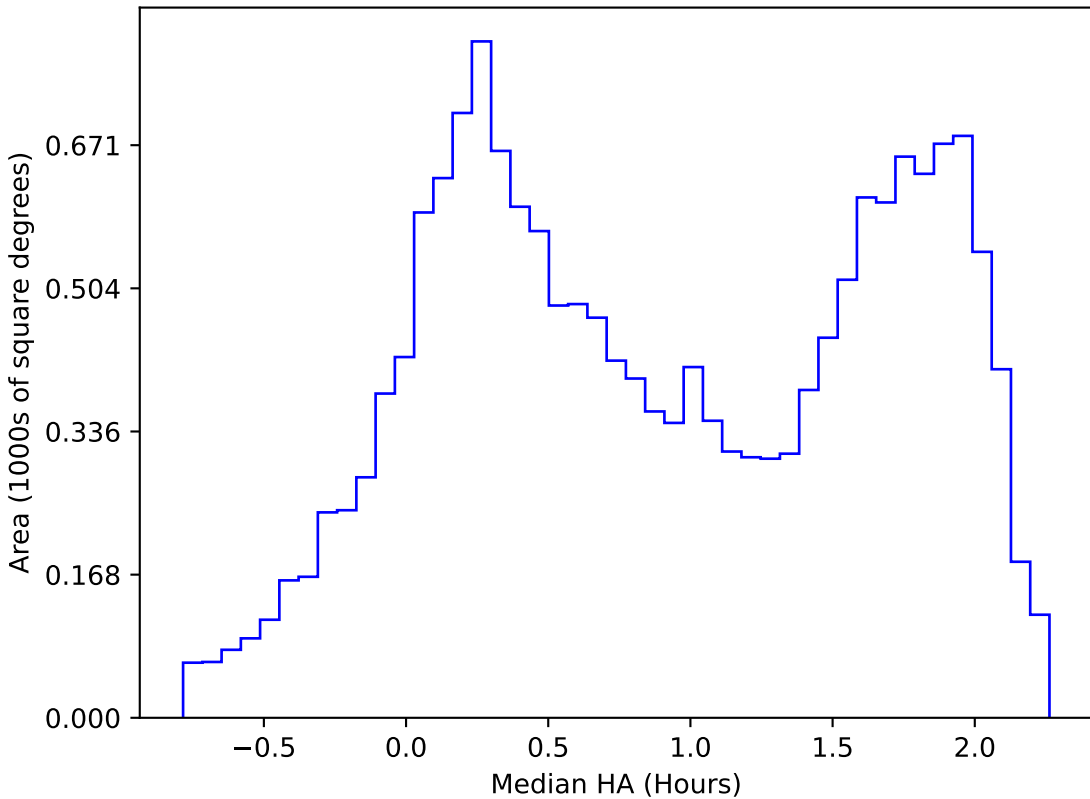
too_elab_r64_d2_griz_v3.4_10yrs WFD r band: Median HA
