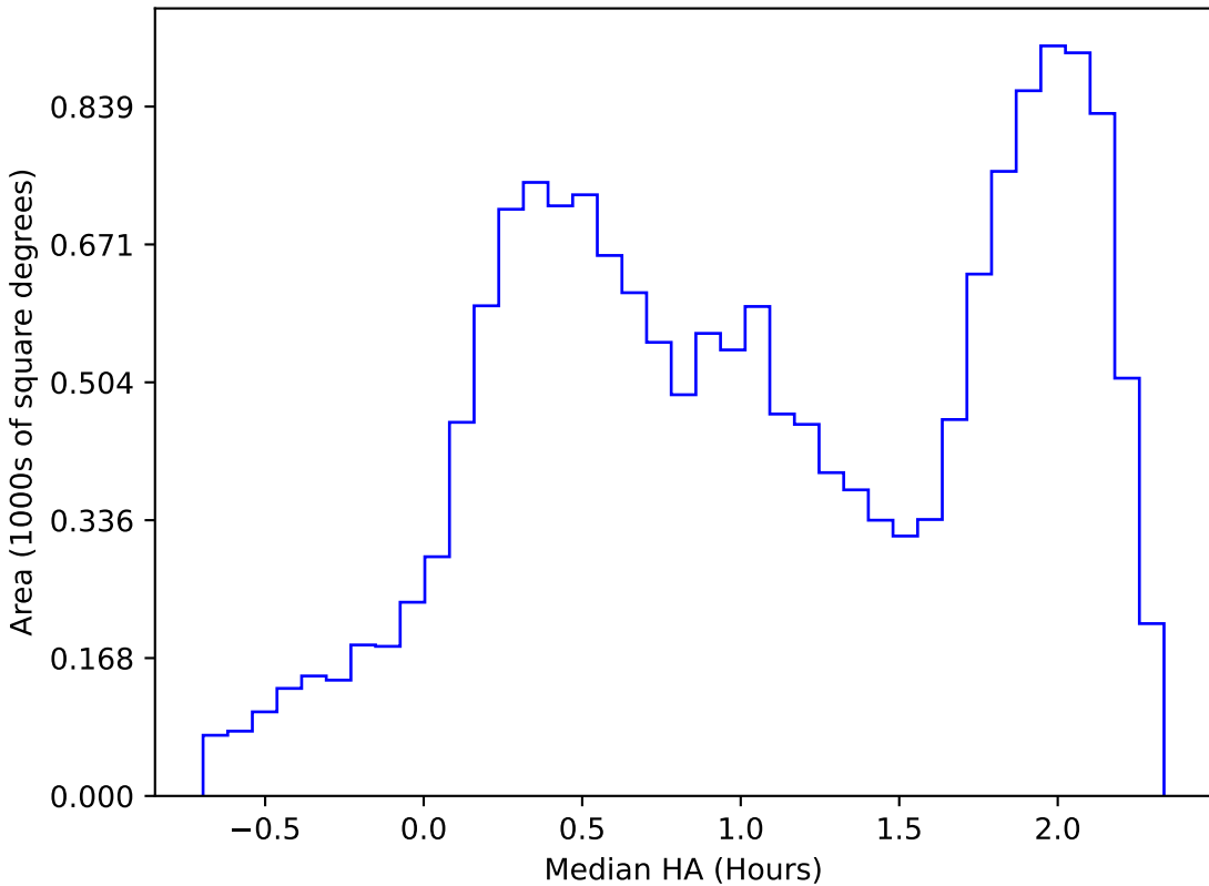
too_elab_r64_d2_griz_v3.4_10yrs WFD i band: Median HA
