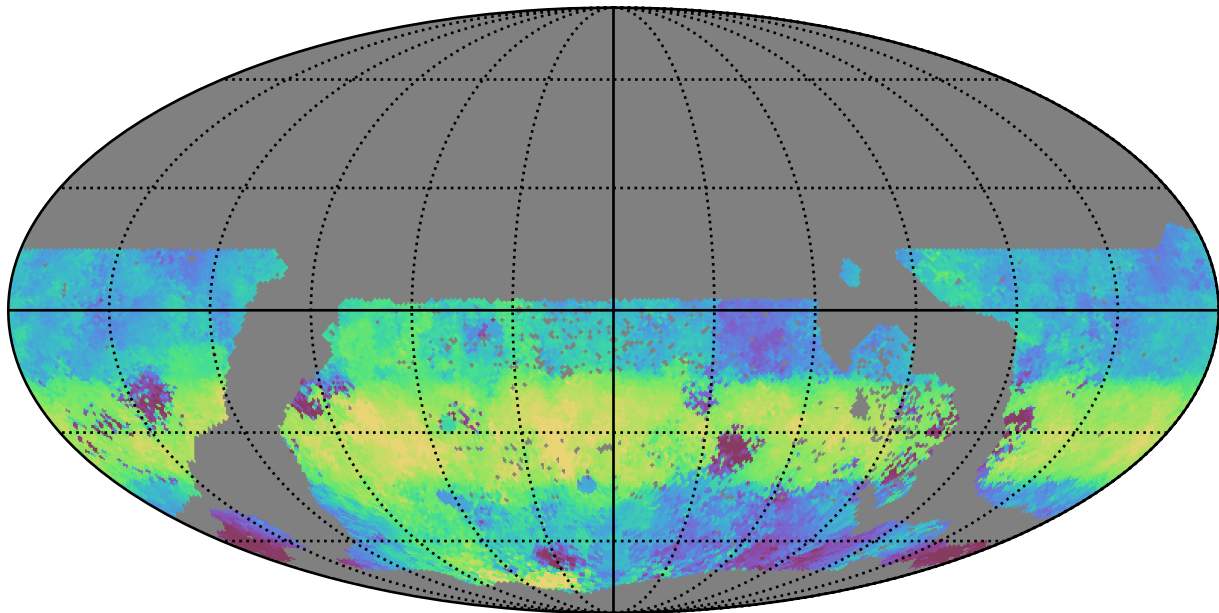
too_elab_r64_d2_griz_v3.4_10yrs WFD g band: Median HA
