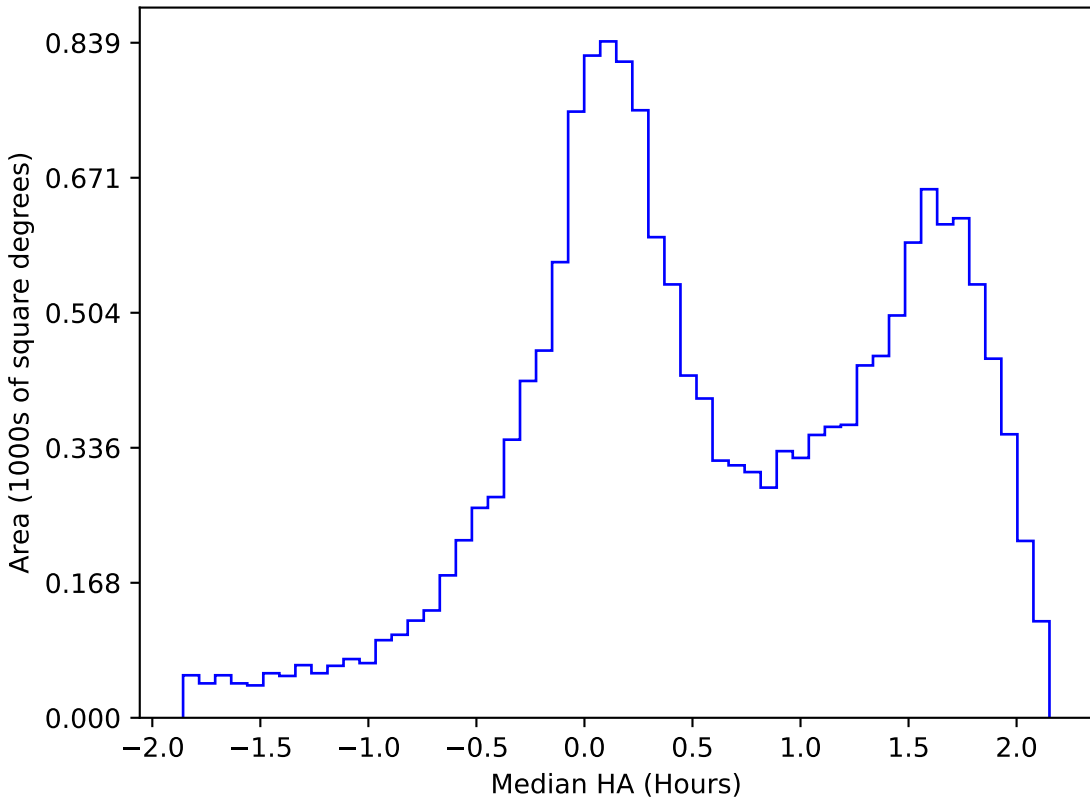
too_elab_r64_d2_griz_v3.4_10yrs WFD g band: Median HA
