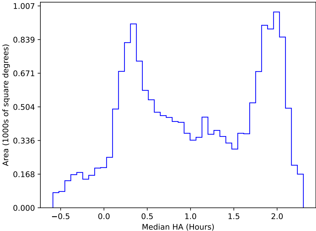
too_elab_r64_d2_griz_v3.4_10yrs WFD all bands: Median HA
