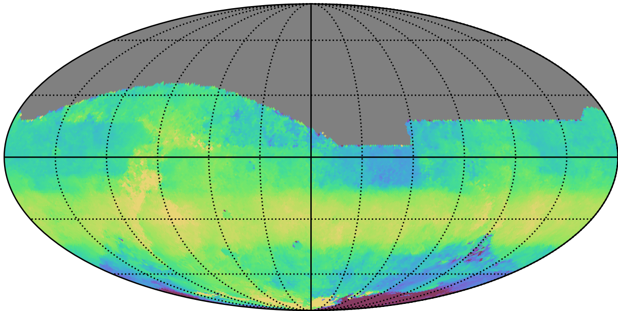
too_elab_r64_d2_griz_v3.4_10yrs All sky z band: Median HA
