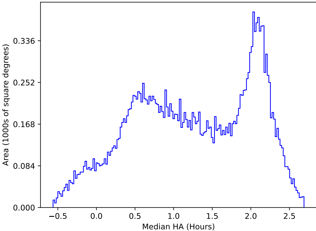
too_elab_r64_d2_griz_v3.4_10yrs All sky y band: Median HA
